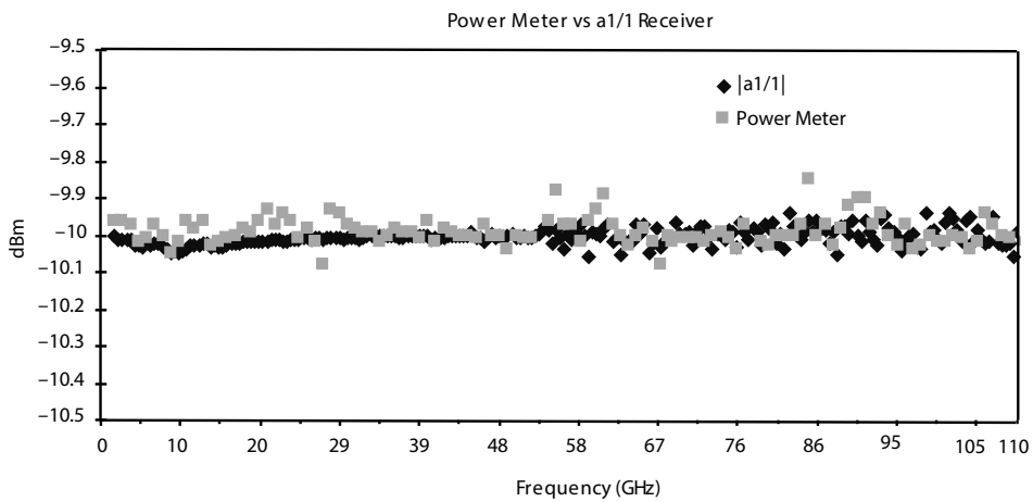
An example of typical power measurement agreement: power sensor vs. ME7838EX a1 reference receiver.
